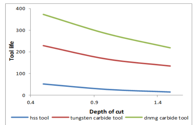
Figure 4c. Effect of depth of cut on life of tools at constant spindle speed of 1400 rev/min
