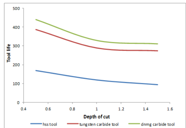
Figure 10c. Effect of depth of cut on life of tools at constant spindle speed of 1400 rev/min
