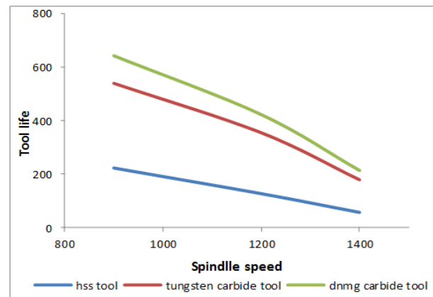
Figure 5c. Effect of spindle speed on life of tools at constant feed rate of 0.3 mm/rev
