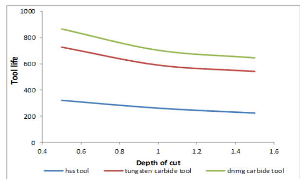
Figure 7a. Effect of depth of cut on life of tools at constant spindle speed of 900 rev/min
