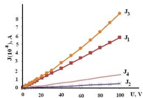
Fig. 6. VAC of Cd_{1-x}Mn_xTe ( x = 0.05 ) thin films obtained on mica substrates: J_1 -before irradiation, J_2 -after irradiation D_\gamma=10krad , J_3 - after irradiation D_\gamma=31krad , J_4 -after irradiation D_\gamma=51krad
