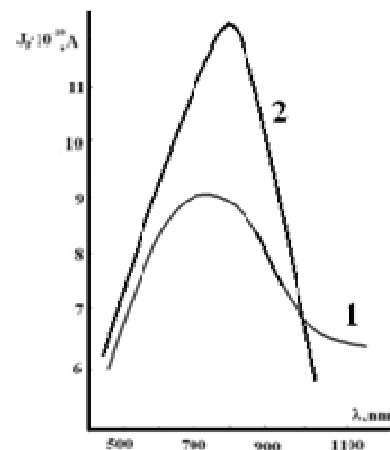
Fig. 7. Photoconductivity of Cd_{1-x}Mn_xTe ( x = 0.05 ) thin films obtained on mica substrate: 1-before irradiation, 2-after irradiation D_\gamma=10krad
