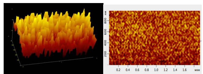
Fig. 4. AFM images of Cd_{1-x}Mn_xTe ( x=0.05 ) thin film
