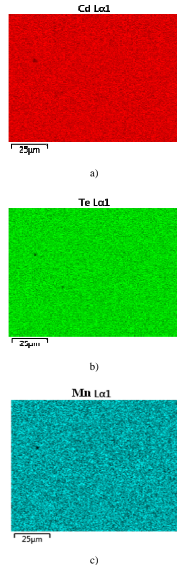
Fig. 3. Elemental Analysis of Cd_{1-x}Mn_xTe ( x=0.05 ) thin film: a) Cd in the sample content b) Te in the sample content c) Mn in the sample content
