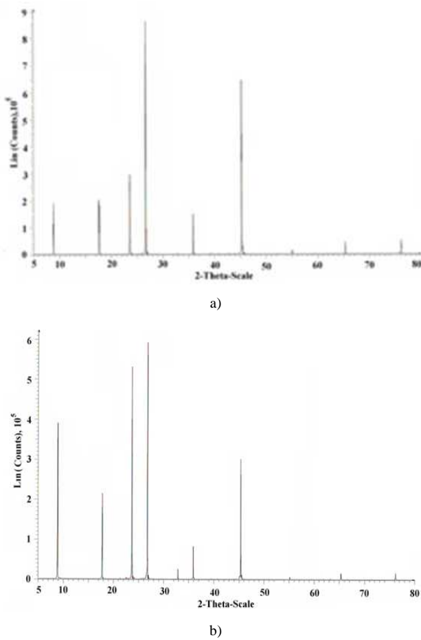
Fig. 5. X-ray diffraction patterns of Cd_{1-x}Mn_xTe ( x=0.05 ) thin films on mica substrate: a) before \gamma -irradiation b) after \gamma -irradiation by E_\gamma=31krad , t_\gamma=23min
